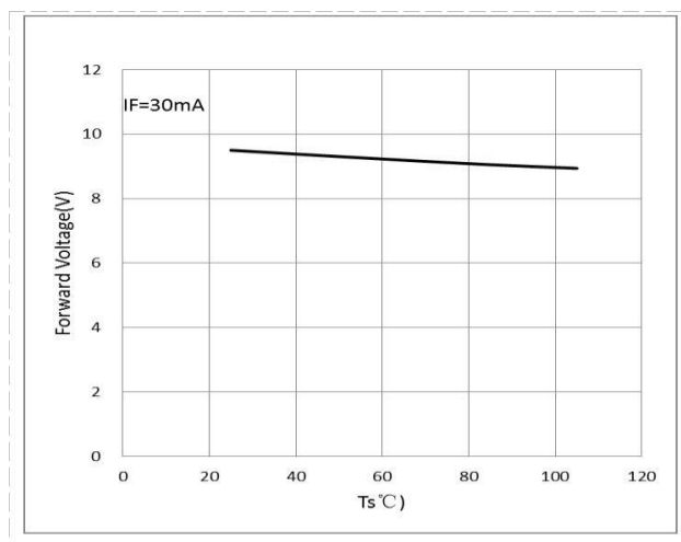
Fig 6. Ambient Temperature vs. Relative Forward Voltage ( I_F=30\text{mA} )
