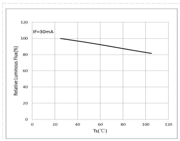
Fig 5. Ambient Temperature vs. Relative Luminous flux ( I_F=30\text{mA} )
