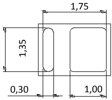
Bot. view
