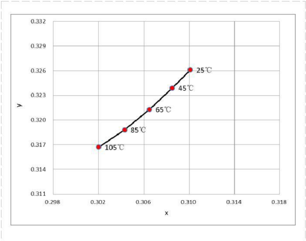
Fig 7. Chromaticity Coordinates vs. Ambient Temperature (IF=30mA)
