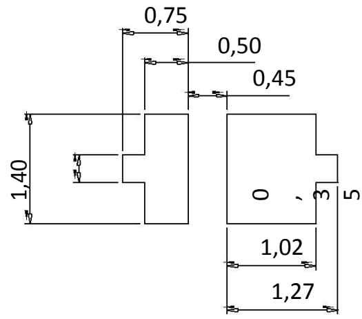
Soldering patterns
